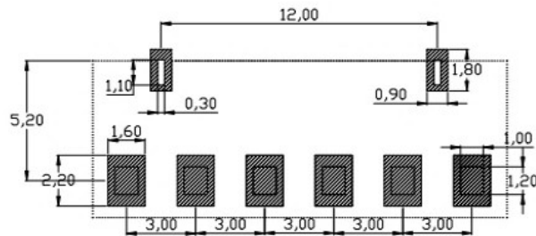
RECOMMENDED PCB LAYOUT TOP VIEW (.XX±0.05)
