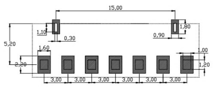
RECOMMENDED PCB LAYOUT TOP VIEW (.XX±0.05)
