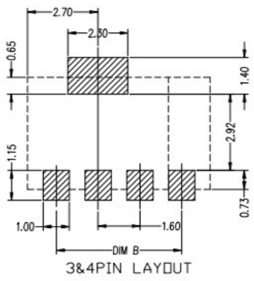
RECOMMENDED PCB LAYOUT TDL(±0.05)
