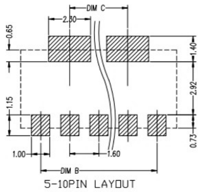
RECOMMENDED PCB LAYOUT TDL(±0.05)
