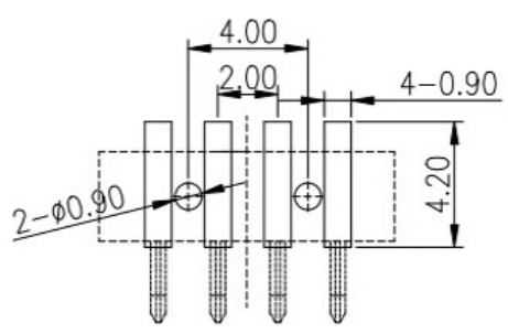
RECOMMENDED P.C.B LAYOUT TOP VIEW (.XX±0.05)
