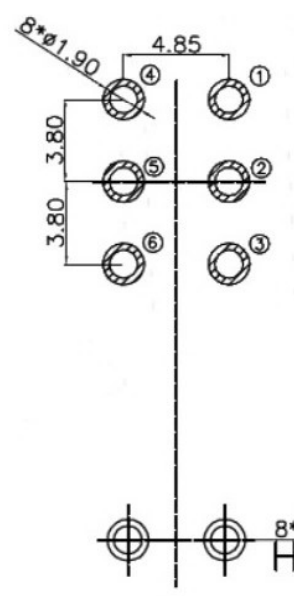
PCB Layout
