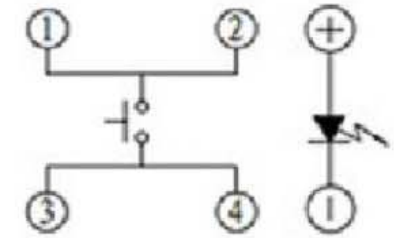
SCHEMATIC
