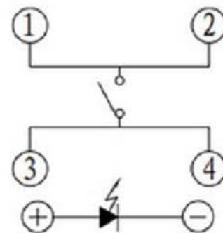
SCHEMATIC
