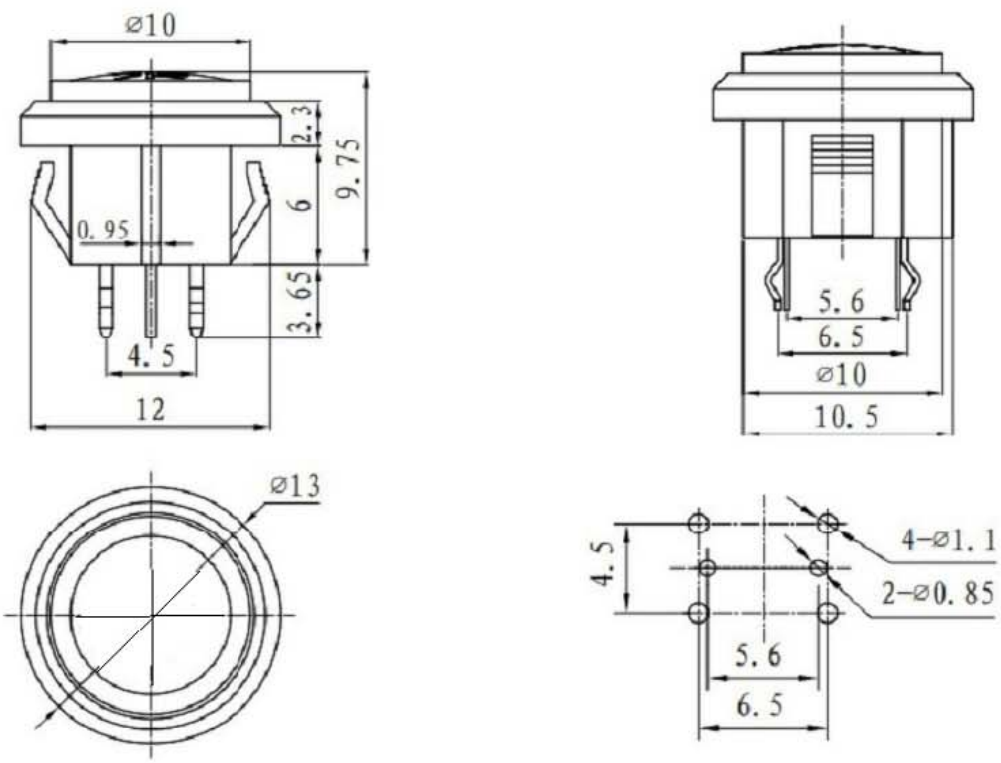
Panel opening (One or two) 面板开孔 (二选一)
