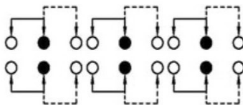
SCHEMATIC (NON-SHORTING)
