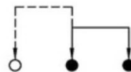
SCHMATIC (NON-SHORTING)
