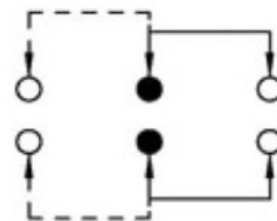
SCHEMATIC (NON-SHORTING)
