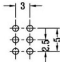
P.C.B LAYOUT BOTTOM VIEW
