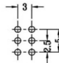
P.C.B. LAYOUT BOTTOM VIEW
