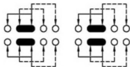
SCHMATIC (SHORTING)
