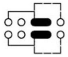
SCHEMATIC (NON-SHORTING)
