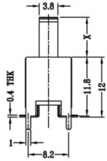
SCHEMATIC (SHORTING)
