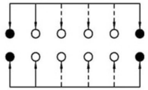
SCHEMATIC (NON-SHORTING)
