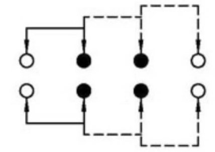
SCHEMATIC (NON-SHORTING)
