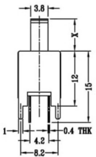
SCHMATIC (SHORTING)
