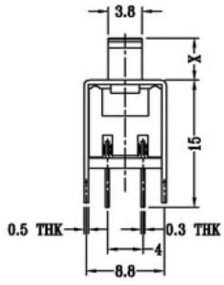
SCHEMATIC (NON-SHORTING)
