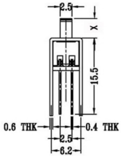
SCHEMATIC (NON-SHORTING)
