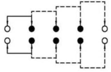
SCHEMATIC (NON-SHORTING)
