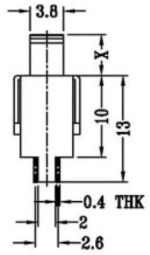
SCHEMATIC (NON-SHORTING)
