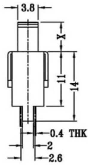
SCHEMATIC (NON-SHORTING)
