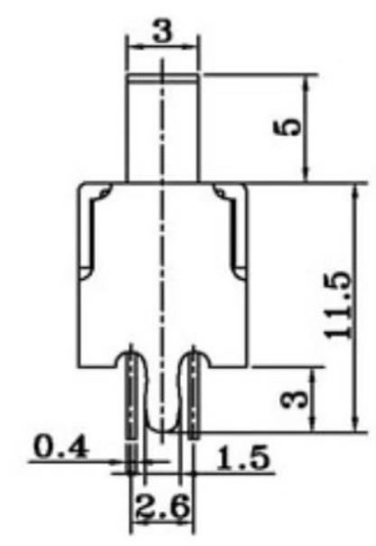
SCHMATIC (NON-SHORTING)
