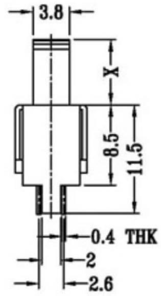
SCHEMATIC (NON-SHORTING)
