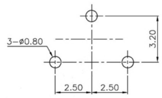
HOLE LAYOUT
