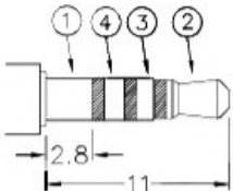
ø2.5mm SPECIAL MATE PLUG
