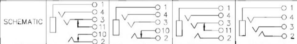
ø2.5mm SPECIAL MATE PLUG
