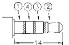
∅3.5 MATE PLUG
