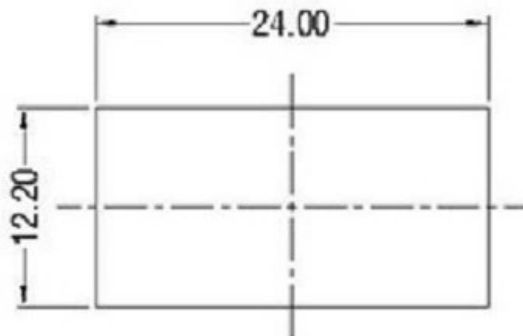
PANEL CUT-OUT
