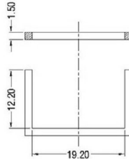
PANEL CUT-OUT
