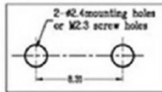
7. Mounting Holes
