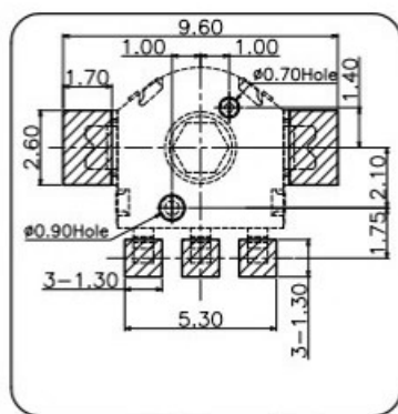
Recommended PCB Layout (Pattern side) tolerance: +/-0.05mm
