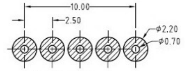
Recommended pin layout Layout tolerance: ±0.05mm
