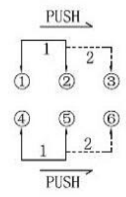
SCHEMATIC (NON-SHORTING)
