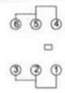
SCHEMATIC (NON-SHORTING)
