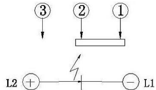
SCHEMATIC (NON-SHORTING)
