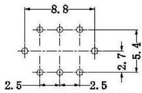
P. C. B LAYOUT
