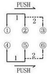
SCHEMATIC (NON-SHORTING)
