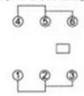
SCHEMATIC (NON-SHORTING)
