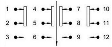
SCHEMATIC (NON-SHORTING)
