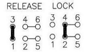
SCHEMATIC (NON-SHORTING)
