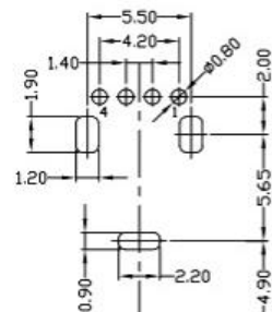
RECOMMEND PCB LAYOUT
