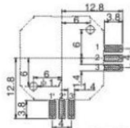
Recommended PAD LAYOUT \pm 0.05 TOP VIEW
