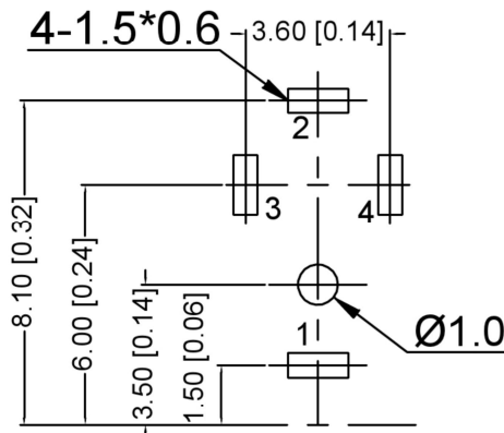
PCB HOLES(TOP VIEW) GENERAL TOLERANCE:0.1MM
