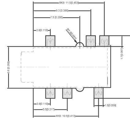
PCB LAYOUT TOP VIEW TOLERANCES:±0.05
