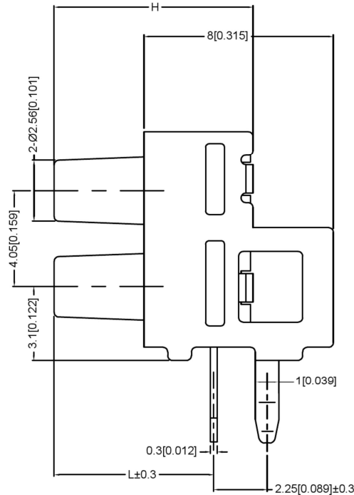
REFERENCE DRAWING
