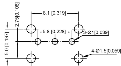
PCB board installation drawing (± 0.1)
