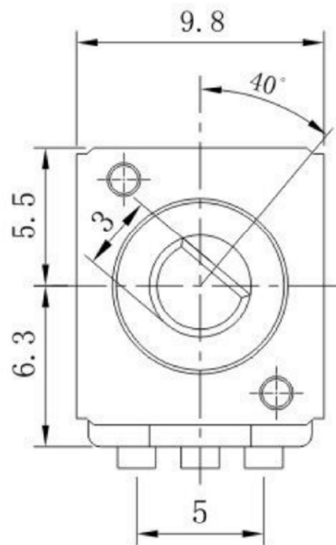
FULL C. C. W POSITION
