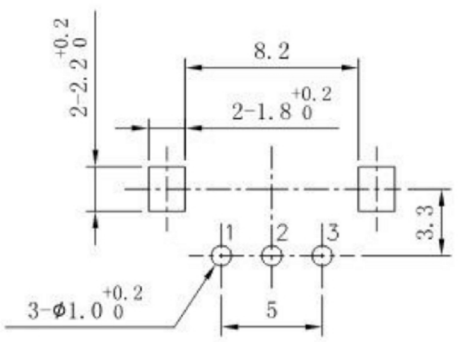
P. C. B MOUNTING HOLE DETAIL
