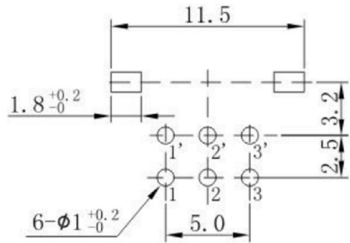
P. C. B MOUNTING HOLE DETAIL
